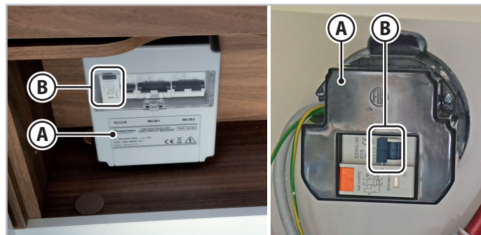
Fig.6.28 - Strømpanel
